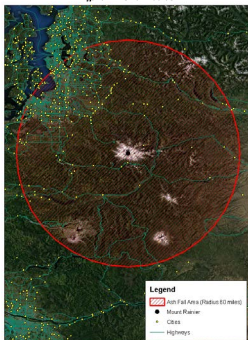
Figure 2 – Ashfall Radius
