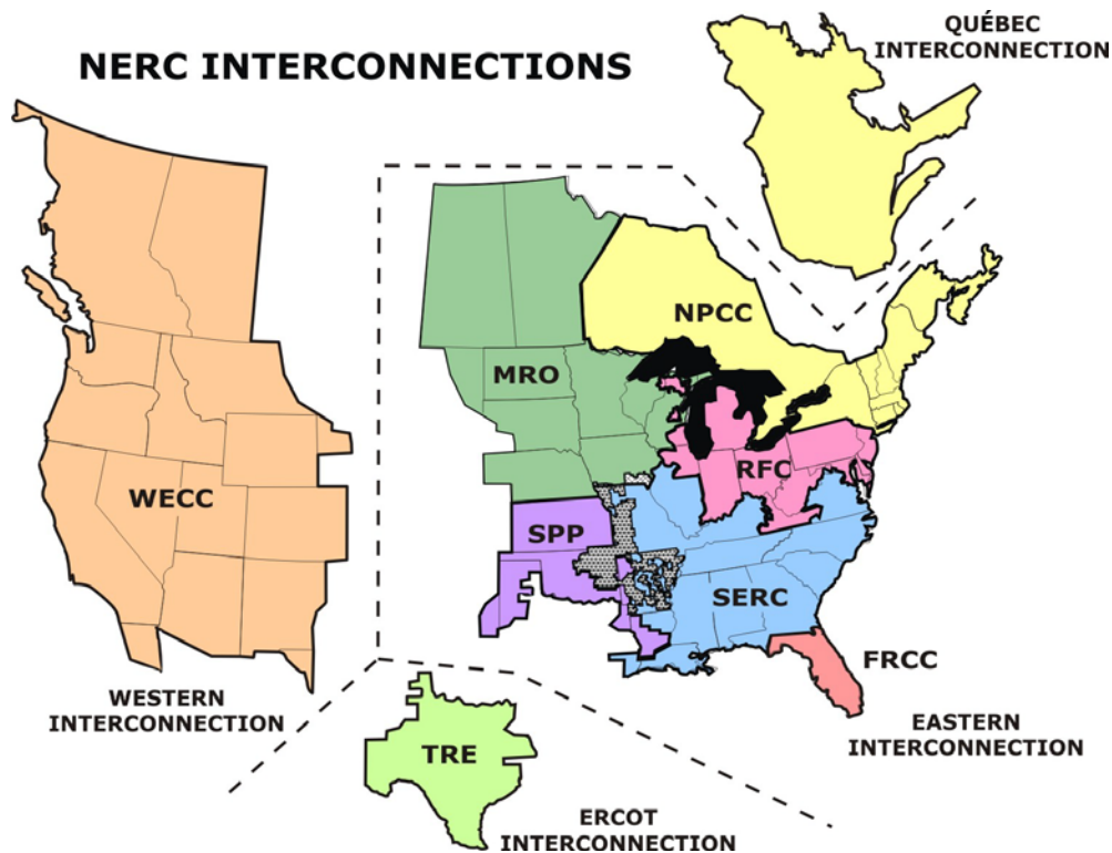
Figure 10: Interconnections and Reliability Regions 39
